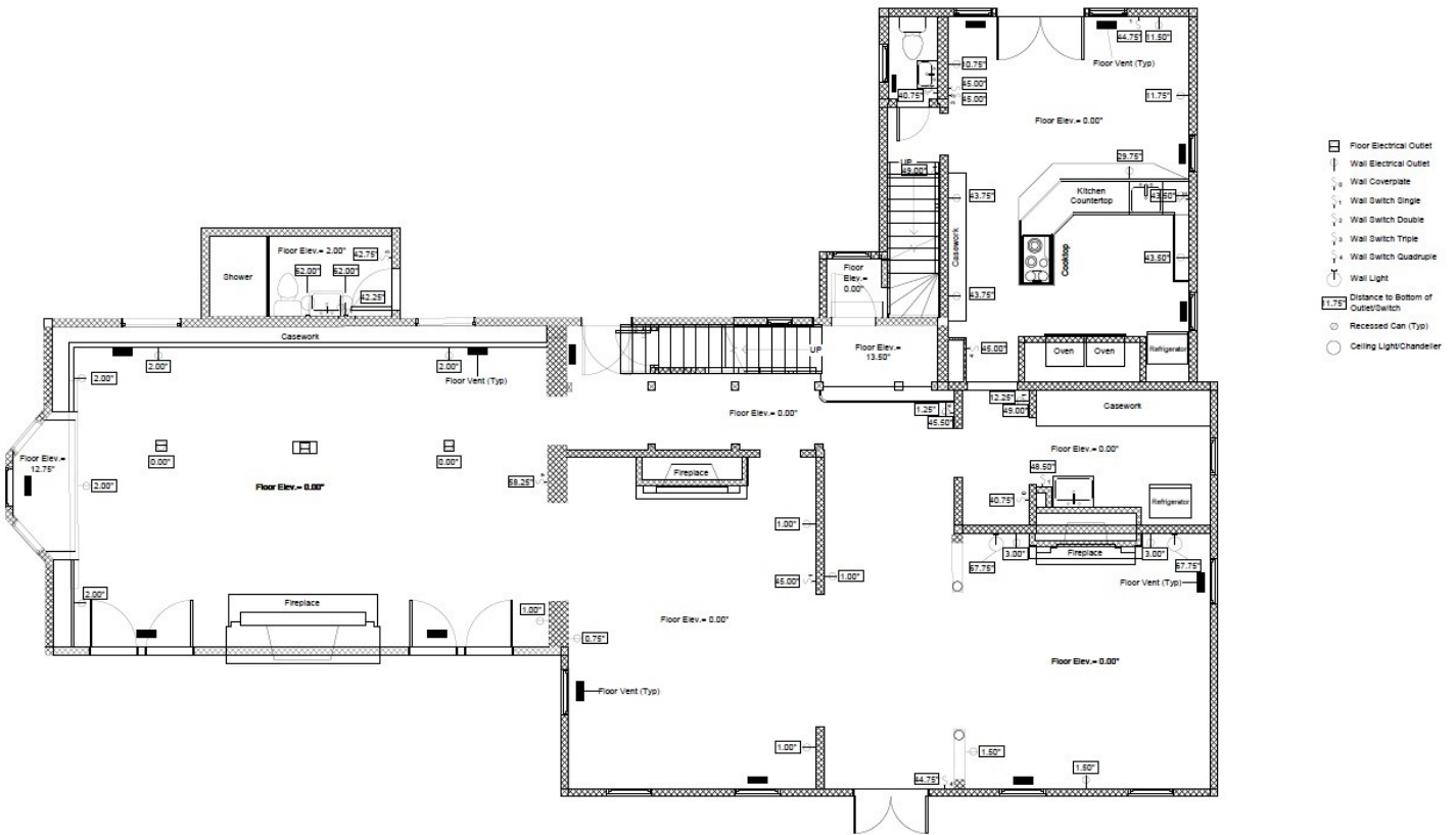
1st Floor Floor Plan
