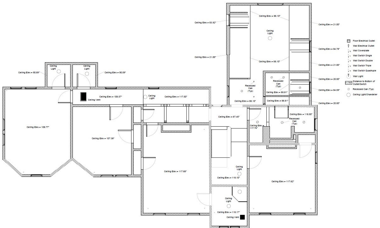
2nd Floor Ceiling Plan
