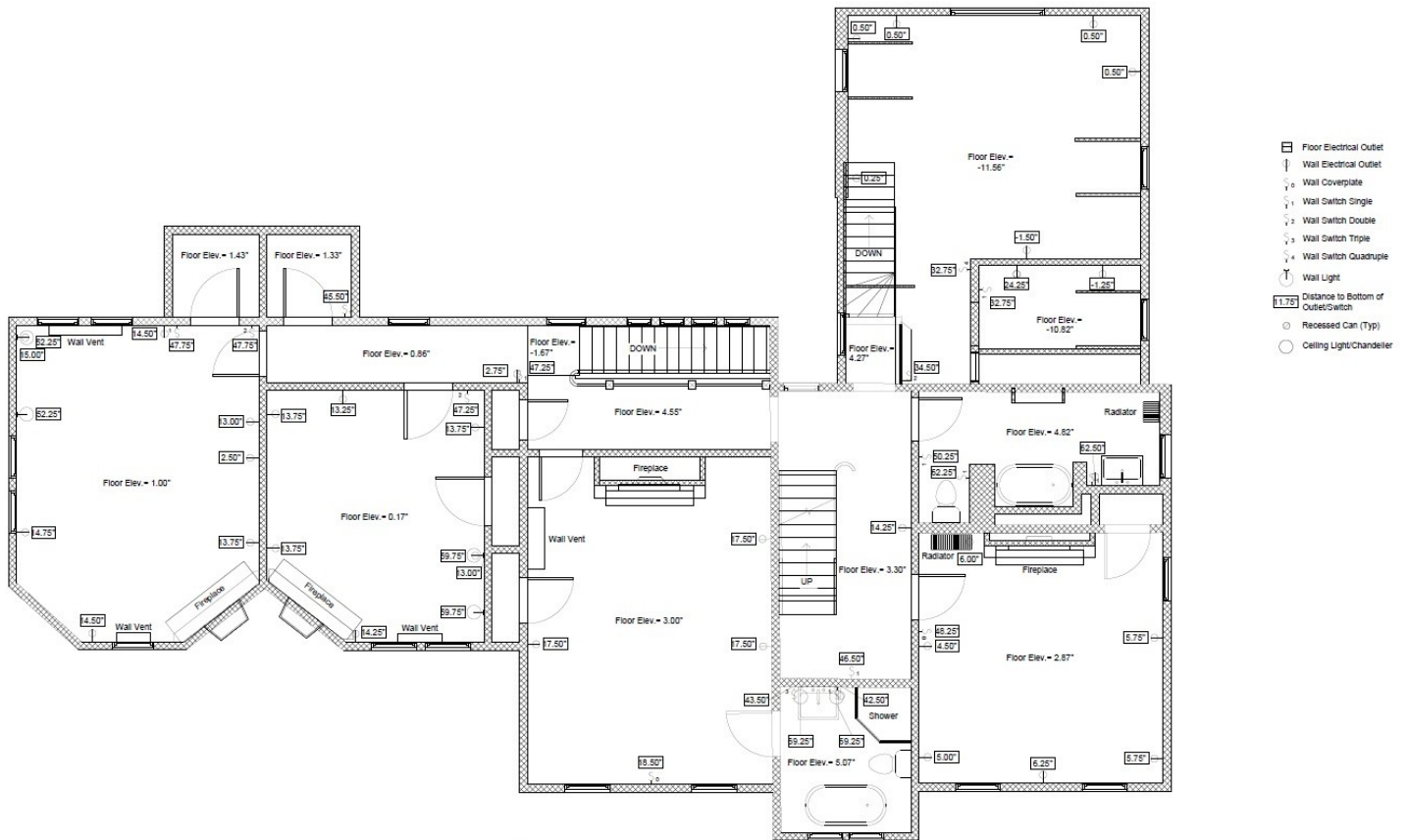
2nd Floor Floor Plan
