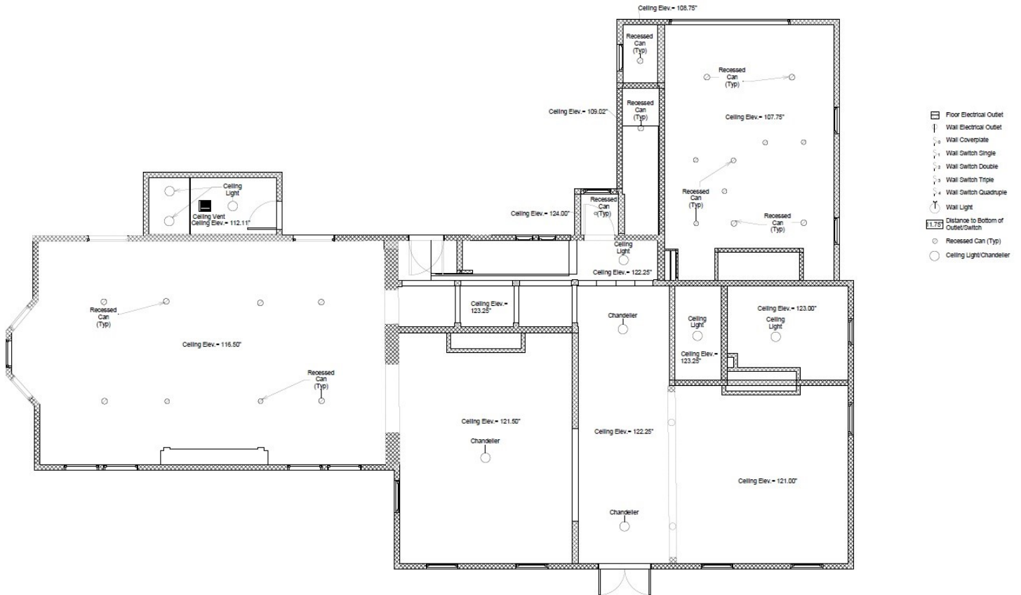
1st Floor Ceiling Plan
